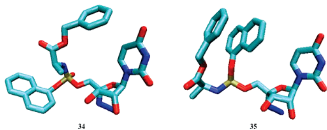
Figure 2. Lowest energy conformations of compounds 34 and 35 .
