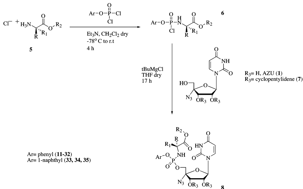
Scheme 1. General Synthetic Pathway for the Synthesis of AZU Aryloxy-phosphoramidates
